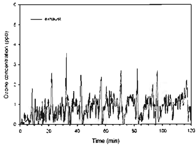
(c) 1,350-time used MPPHS
